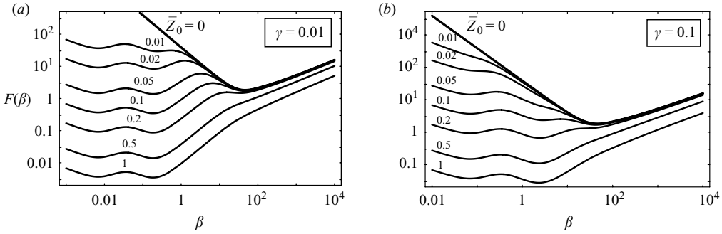
FIGURE 20. Same as figure 19 for \gamma = 0.01, 0.1 .
